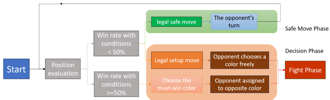
Figure 1. The flowchart of Cusp Chess.
