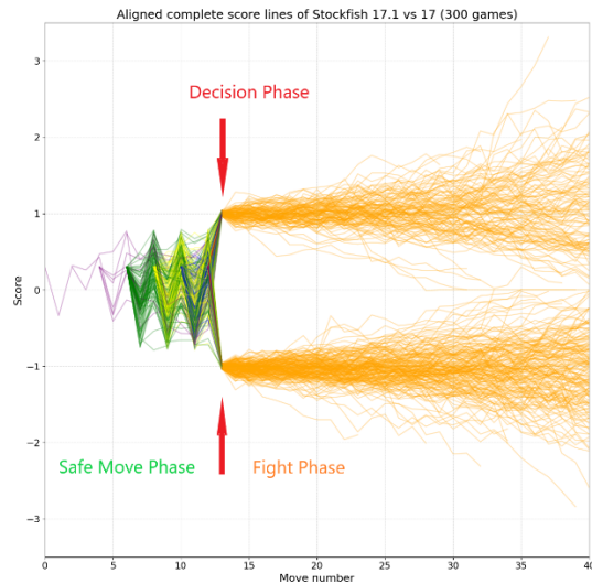
Figure 4. Aligned score lines with extra moves in Fight Phase.
