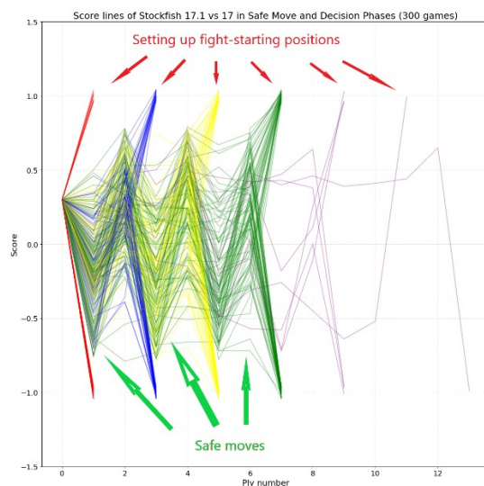
Figure 4. Score lines in Safe Move Phase and Decision Phase.
