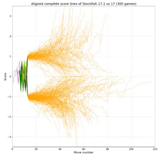
Figure 5. Aligned complete score lines.
